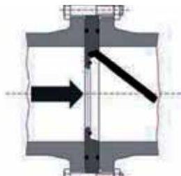
Horizontal flow
